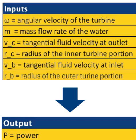
Figure 3: Input and Outputs of Euler’s Turbine Equation
