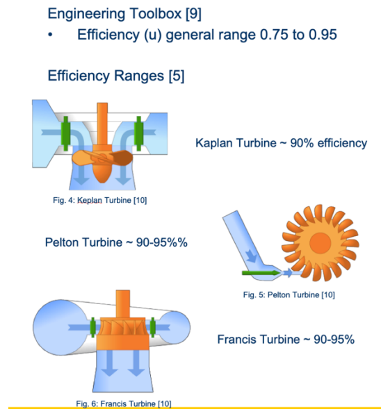
Figure 2: Turbine Types with Efficiency
