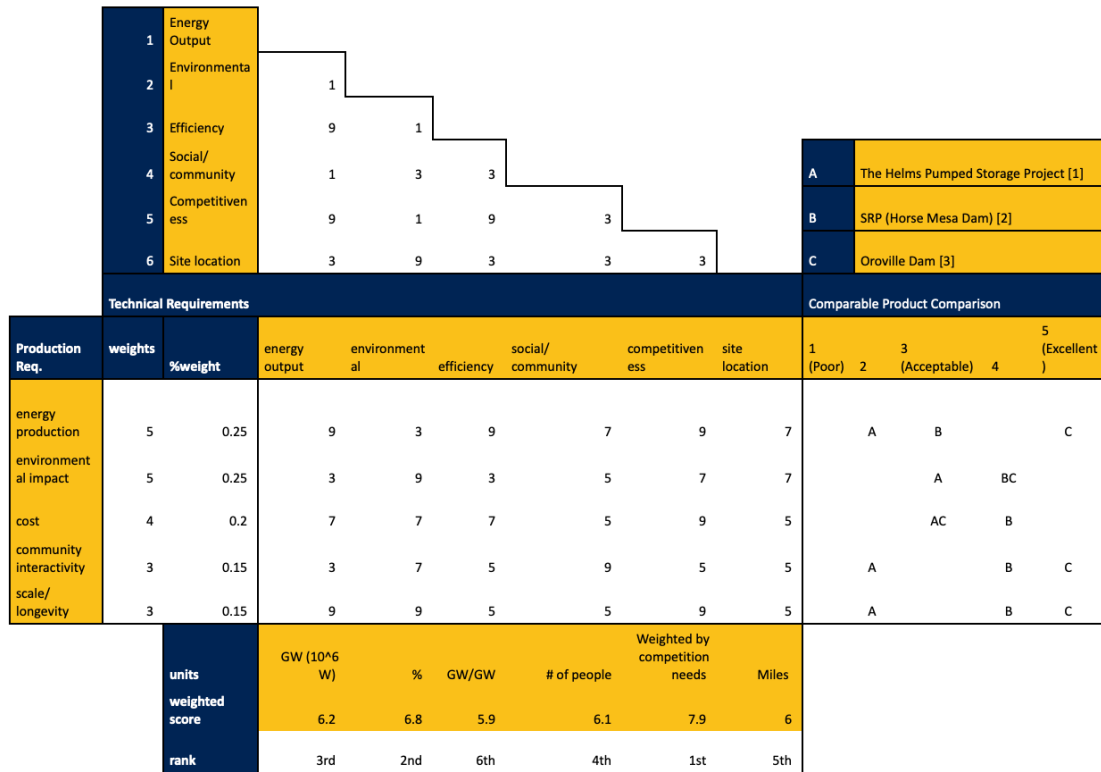
Figure 1: HoQ
