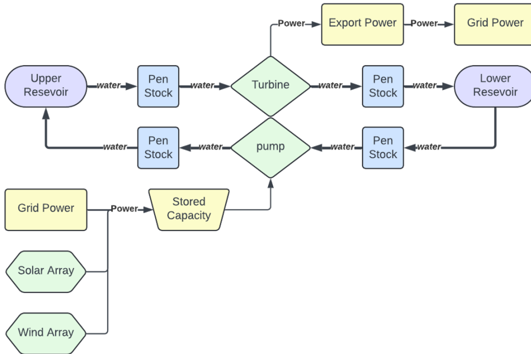
Figure 9: Functional Model
